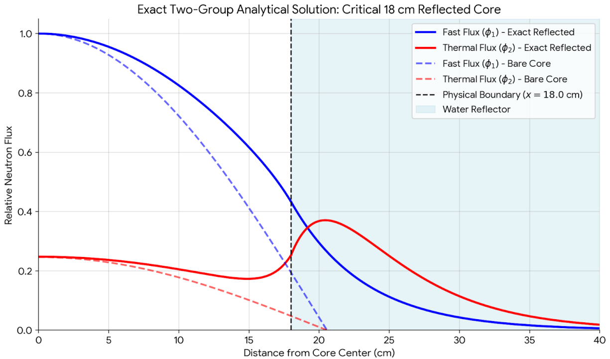
Figure 2: Exact two-group analytical flux distributions for an 18 cm core, comparing bare versus water-reflected boundary conditions. Note the localized thermal flux peak in the reflector region and the precise transient "hook" representing inward backward diffusion at the core periphery.
